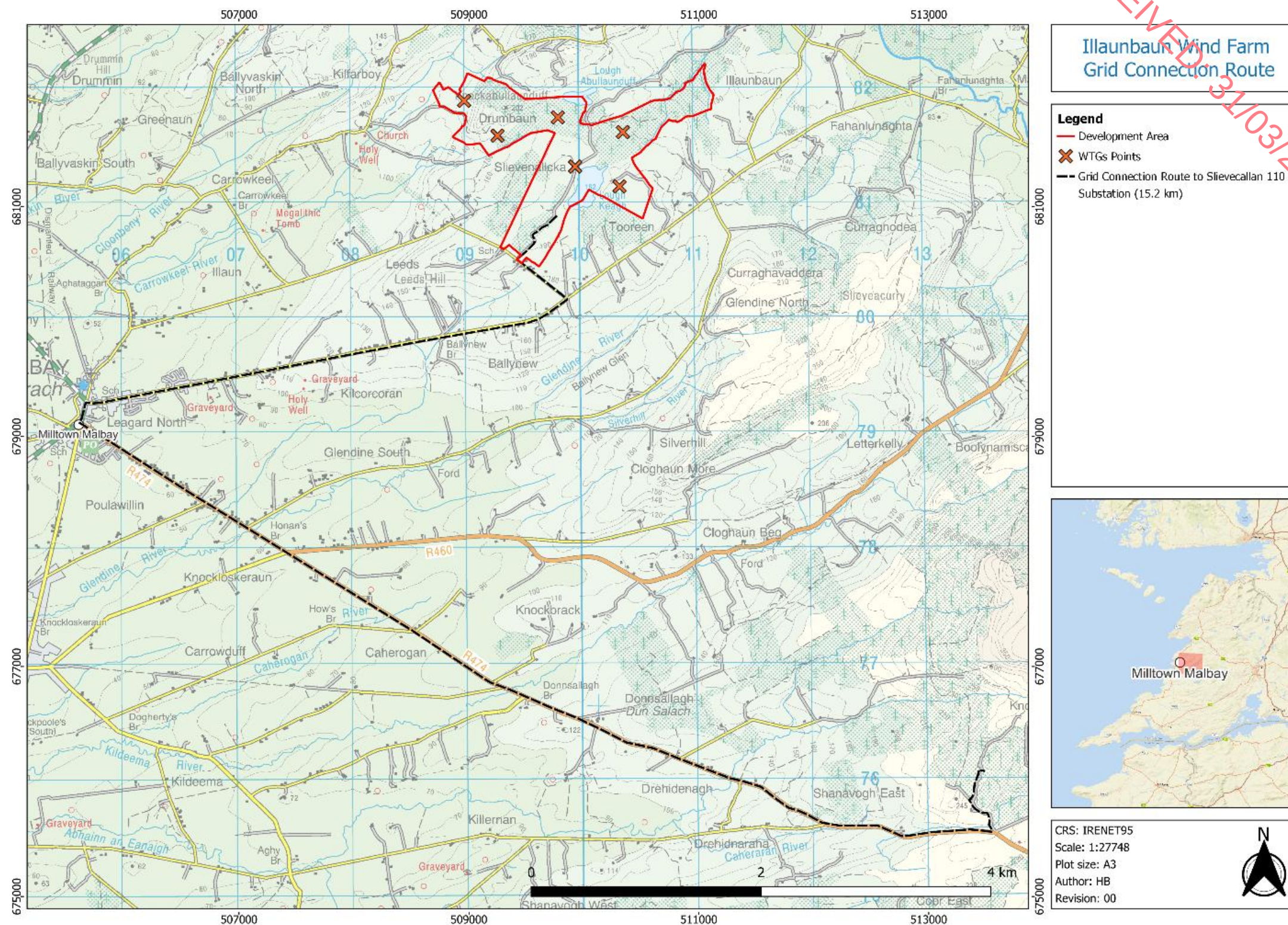
Figure 1-2: Anticipated Grid Connection Route
