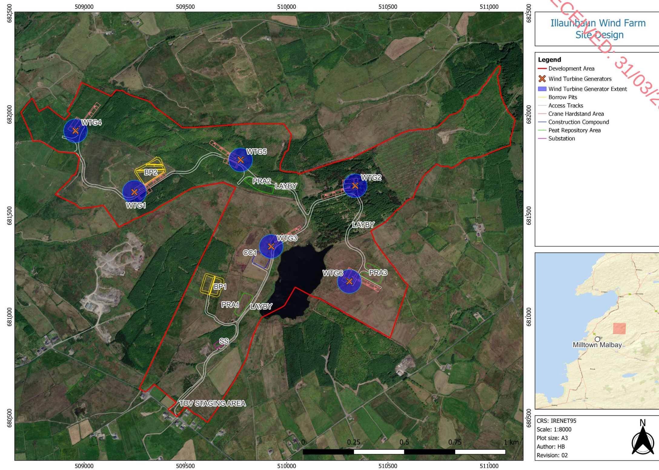
Figure 1-1: Site Layout Plan (with Slievenalicka Wind Turbine indicated as WTG4)
